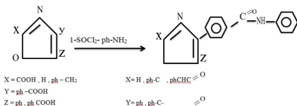
Figure 1: Preparation of Amides
