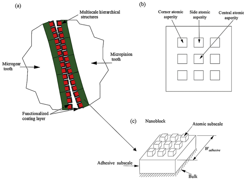
Fig. 4. Hierarchically organised multiscale asperities over the surface of microgear tooth: a) a silicon microgear tooth (gray) is covered by adhesive layer (green) with superimposed atomic scale asperities (red), and the whole structure is covered by an OTS-SAM coating layer (black); b) a plane view of a nano-block covered by atomic scale asperities; c) a nanoblock representing a MEMS asperity. (For interpretation of the references to colour in this figure legend, the reader is referred to the Web version of this article.)
