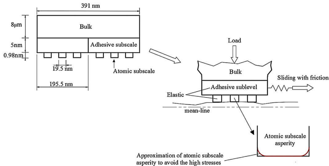
Fig. 8. Approximation of geometry shape for the atomic subscale asperities.
