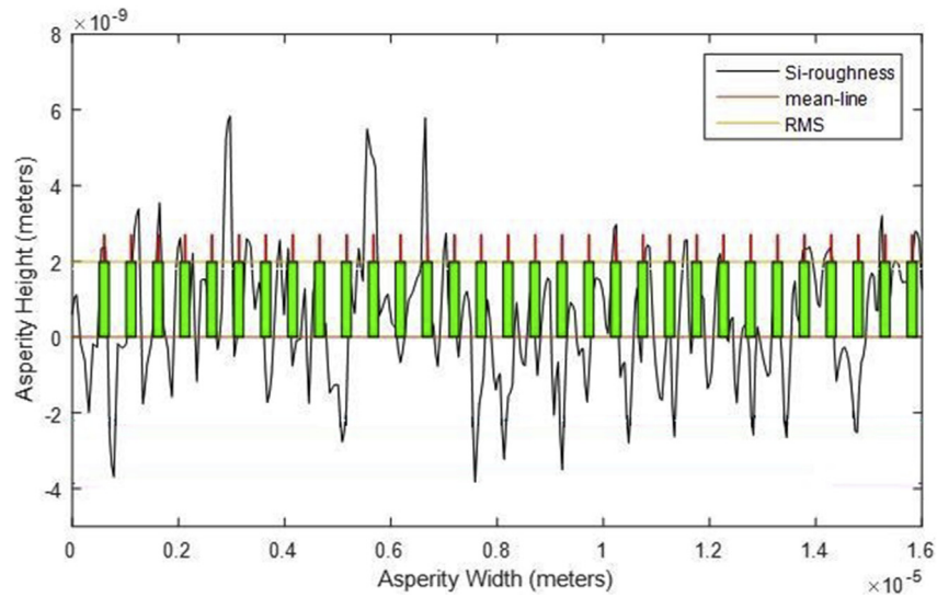
Fig. 2. Computation of the width of the chemical and the van der Waals (green zones) interaction subscales for silicon roughness profile. (For interpretation of the references to colour in this figure legend, the reader is referred to the Web version of this article.)
