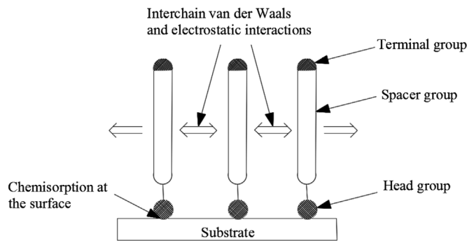
Fig. 1. Self-assembled monomolecular layer on a silicon substrate and the corresponding intermolecular forces (adapted from Ref. [9]). (For interpretation of the references to colour in this figure legend, the reader is referred to the Web version of this article.)
