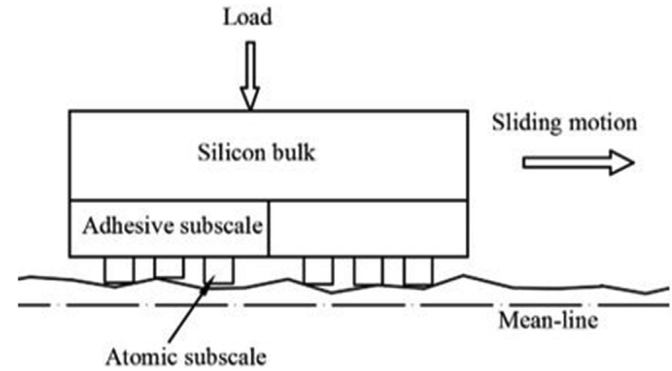
Fig. 3. A multi-scale hierarchical structure with a vertical degree of freedom.
