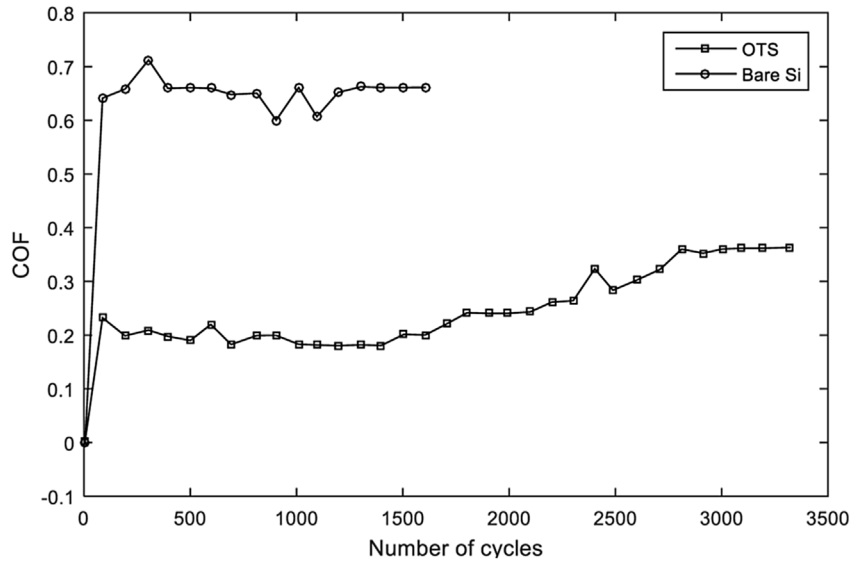
Fig. 6. Experimental results on variation of COF with sliding cycles for bare Si and OTS at a sliding velocity of 2 cm/s and normal load of 5 g m [45].
