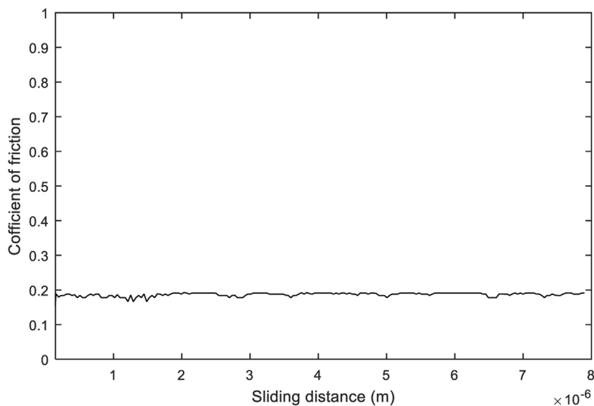
Fig. 5. Numerical results on variation of COF for functionalized coating teeth surface by OTS-SAM layer [22].
