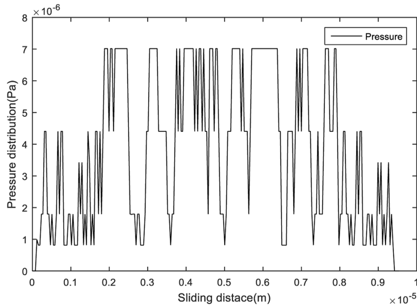
Fig. 10. Distribution of pressure acting on a tooth along x (sliding distance). There are k = 48 picks of the pressure fluctuations.
