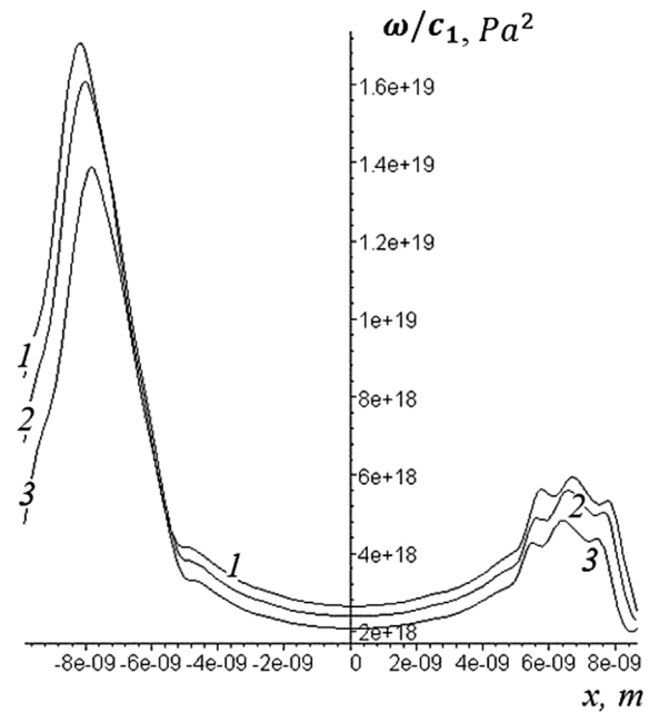
Fig. 14. Damage function ( \omega/c_1 ) when m = 2 , corner atomic subscale asperity (line 1), side atomic subscale asperity (line 2) and central atomic subscale asperity (line 3) respectively.
