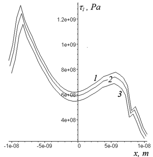
Fig. 11. Principal shear stress distributions for corner (1), side (2) and central atomic subscale asperities (3) when load is maximum 7.016 \times 10^{-6} N .
