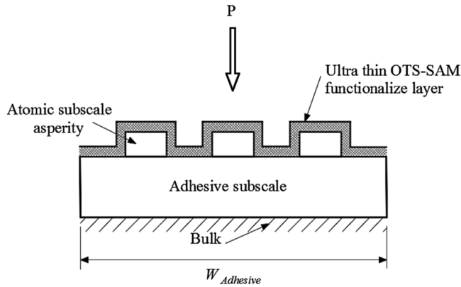
Fig. 7. A nanoblock functionalized by carbon-based monomolecular layer.
