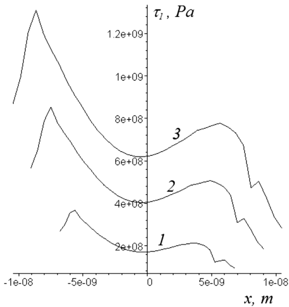
Fig. 12. Principal shear stress distributions for the corner atomic subscale asperity with different values of load ( 0.816 \times 10^{-6}N , 3.428 \times 10^{-6}N and 7.016 \times 10^{-6}N for lines 1, 2 and 3 respectively).
