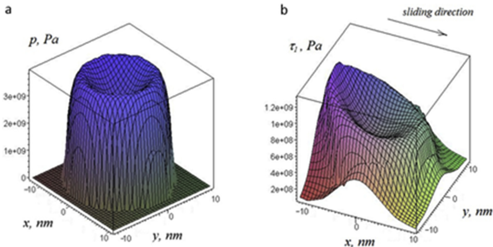
Fig. 9. (a) Contact pressure for atomic subscale asperity; (b) principal shear stress \tau at the surface of atomic subscale asperity.
