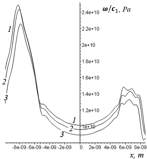
Fig. 13. Damage function ( \omega/c_1 ) when m = 1 , corner atomic subscale asperity (line 1), side atomic subscale asperity (line 2) and central atomic subscale asperity (line 3) respectively.
