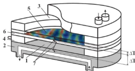
Fig. 1 Convection chamber: 1 – nanofluid; 2,3 – copper and plexiglass heat exchangers; 4 – annular frame; 5 – thermal sensitive liquid – crystalline film; 6 – protective plate; 7 – thermocouples
