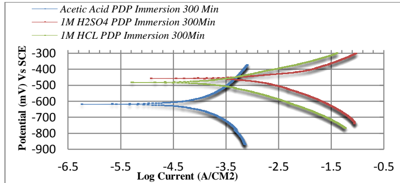
Figure (4) Carbon Steel Immersion in three acidic solutions for 300min
