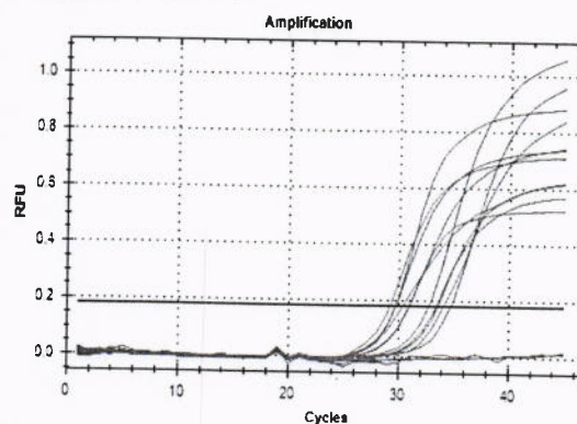
Fig. (1): Amplification plot of Y. enterocolitica attachment invasion locus protein ( ail ) gene by Real-Time PCR in some type of foods.
