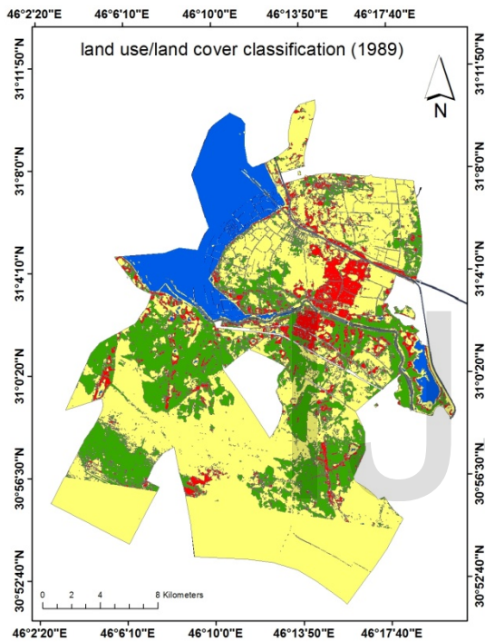
Fig. : 3 land use/land cover classification at 1989
