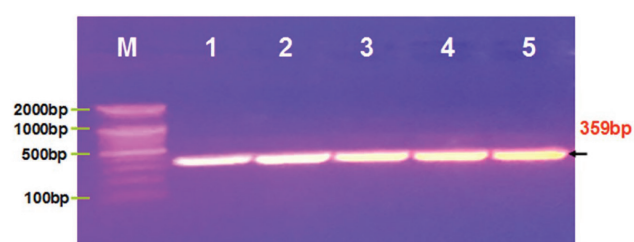
Fig. 4 Agarose gel electrophoresis image that show the PCR product 359-bp analysis of CHY2. Where M: marker (100–2000 bp), lane 1: C. albicans ; lane 2: T. rubrum ; lane 3: M. canis ; lane 4 and 5: A. niger ; lane 5: C. albicans standard strain (ATCC 1032).
