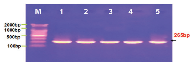
Fig. 2 Agarose gel electrophoresis image that show the PCR product 265 bp analysis of CRD1. Where M: marker (100–2000 bp), lane 1: C. albicans ; lane 2: T. rubrum ; lane 3: M. canis ; lane 4 and 5: A. niger ; lane 5: C. albicans standard strain (ATCC 1032).
