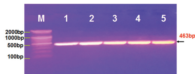
Fig. 1 Agarose gel electrophoresis image that show the PCR product (463 bp) analysis of CHY1. Where M: marker (100–2000 bp), lane 1: C. albicans ; lane 2: T. rubrum ; lane 3: M. canis ; lane 4 and 5: A. niger ; lane 5: C. albicans standard strain (ATCC 1032).
