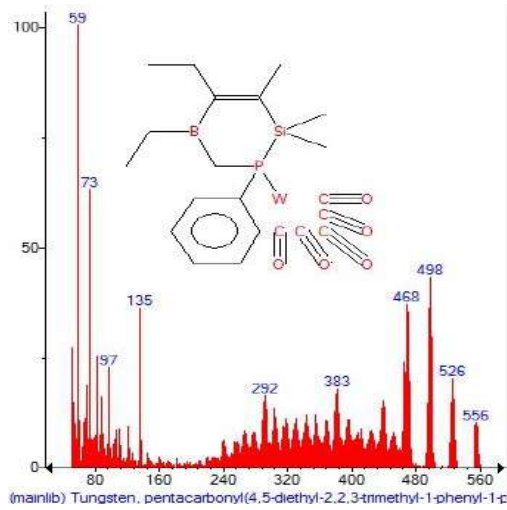
Figure 3: Mass spectrum of Tungsten, pentacarbonyl(4,5-diethyl-2,2,2-trimethyl-1-phenyl-1-c) with Retention Time (RT)= 3.144
