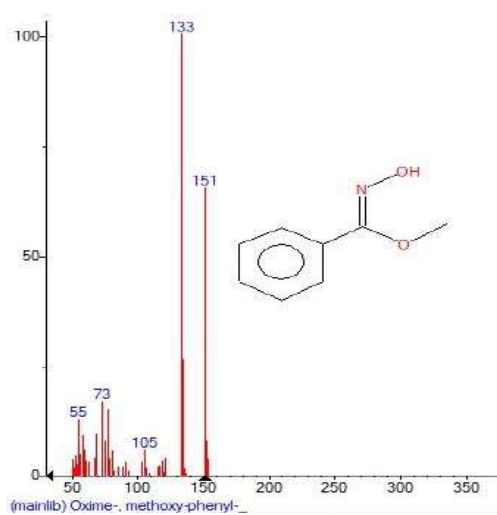
Figure 22: Mass spectrum of Oxime-, methoxy-phenyl- with Retention Time (RT)= 4.678
