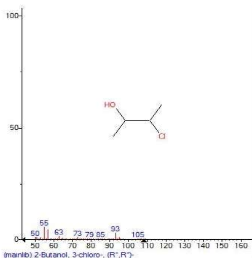
Figure 15: Mass spectrum of 2-Butanol, 3-chloro-, (R*,R*)- with Retention Time (RT)= 3.808
