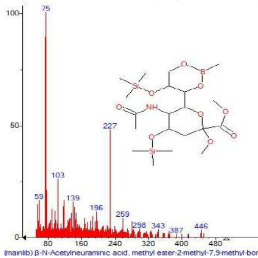
Figure 5: Mass spectrum of \beta -N-Acetylneuraminic acid, methyl ester-2-methyl-7,9-methyl-bor with Retention Time (RT)= 3.276
