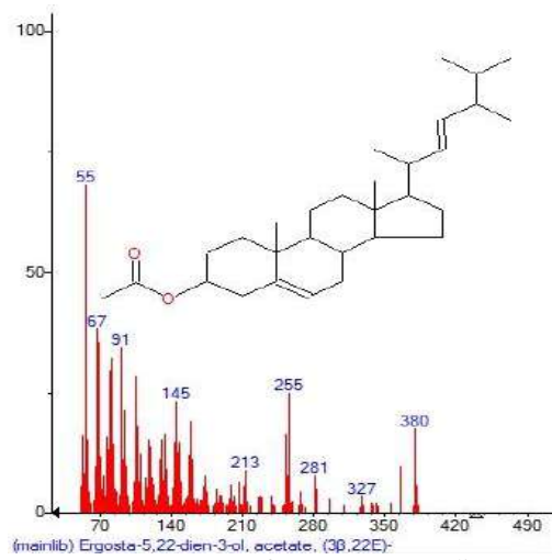
Figure 40: Mass spectrum of Ergosta-5,22-dien-3-ol,acetate,(3β,22E)- with Retention Time (RT)= 8.820
