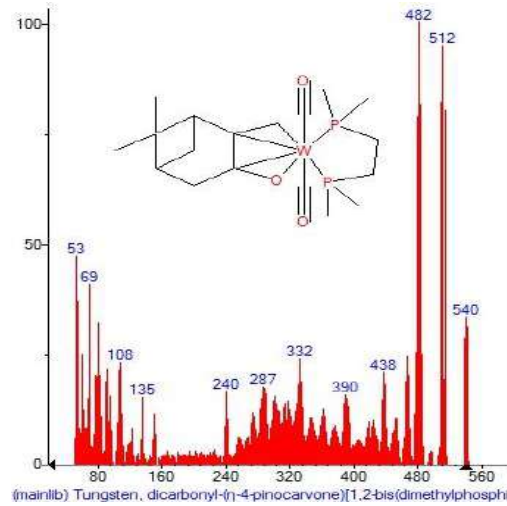
Figure 6: Mass spectrum of Tungsten, dicarbonyl-(n-4-pinocarovone)[1,2-bis(dimethylphosphi with Retention Time (RT)= 3.333
