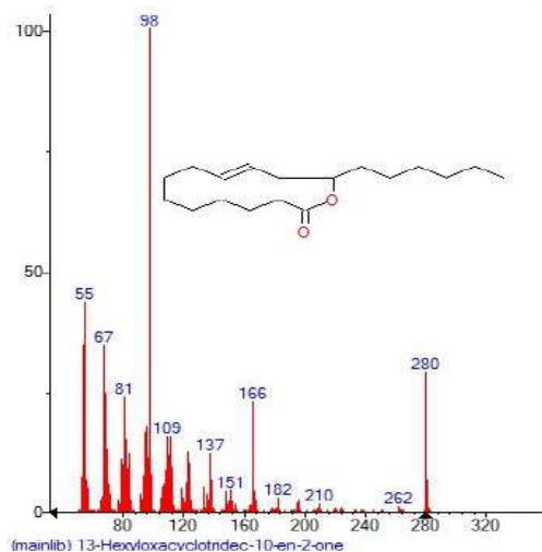
Figure 24: Mass spectrum of 13-Hexyloxacyclotridec-10-en-2-one with Retention Time (RT)= 4.941
