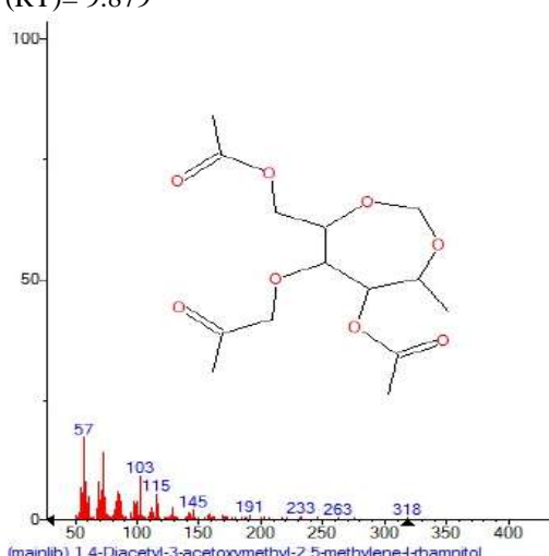
Figure 44: Mass spectrum of 1,4-Diacetyl-3-acetoxymethyl-2,5-methylene-1-rhamnitol with Retention Time (RT)= 11.464
