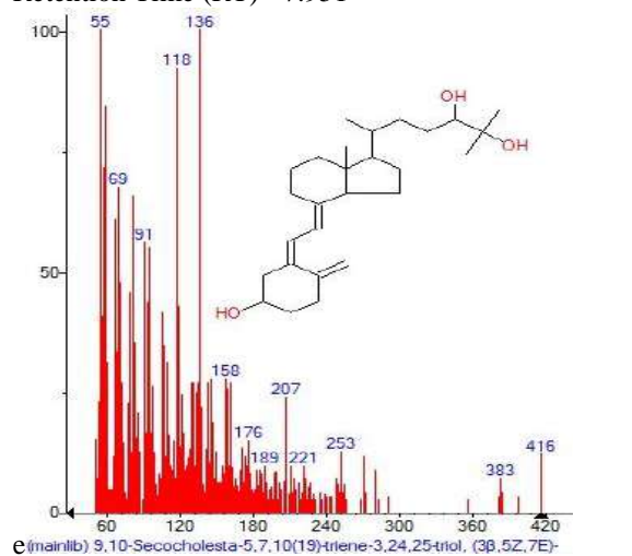
Figure 38: Mass spectrum of 9,10-Secocholesta-5,7,10(19)-triene3,24,25-triol,(3 \beta ,5Z,7E)- with Retention Time (RT)= 8.425
