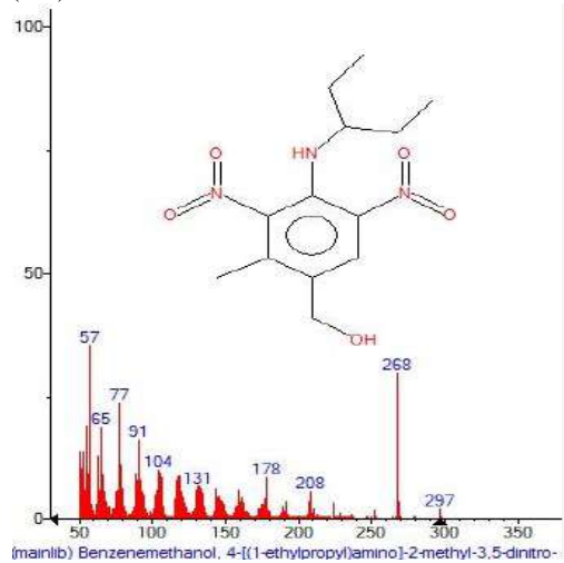
Figure 48: Mass spectrum of Benzenemethanol, 4-[(1-ethylpropyl)amino]-2-methyl-3,5-dinitro- with Retention Time (RT)= 14.708
