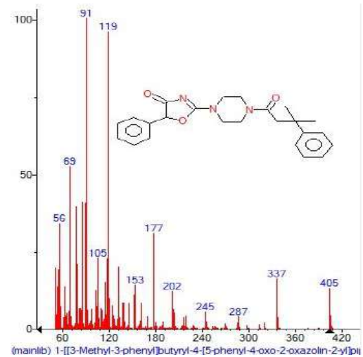
Figure 36: Mass spectrum of 1-[[3-Methyl-3-phenyl]butyryl-4-[5-phenyl-4-oxo-2-oxazolin-2-yl]]l with Retention Time (RT)= 7.951
