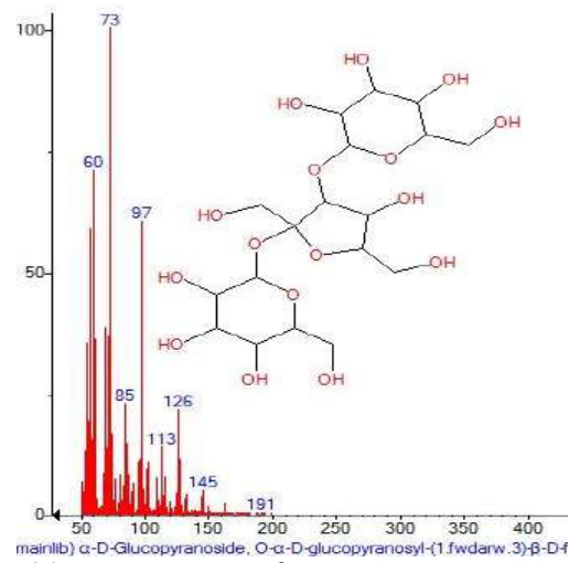
Figure 34: Mass spectrum of \alpha -D Glucopyranoside, O- \alpha -D-glucopyranosyl-(1.fwdarw.3)- \beta - with Retention Time (RT)= 7.373
