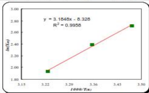
Figure 7: \ln X_m against reciprocal absolute T
