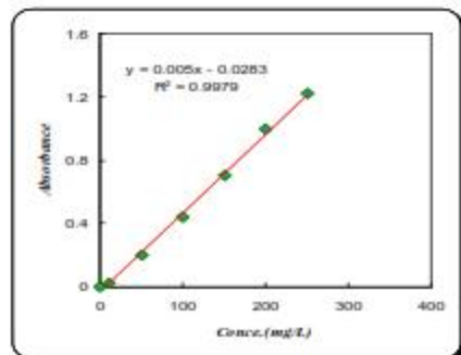
Figure 2: Aspirin calibration curve at \lambda max 275 nm
