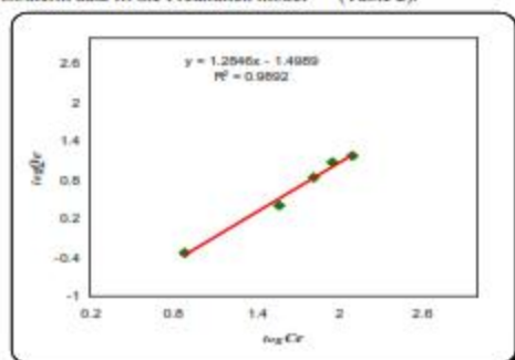
Figure 5: Aspirin Freundlich isotherm on hydrogel
