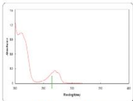
Figure 1: UV spectrum of Aspirin
