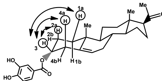
Figure 3. NOESY 1 H, 1 H NMR correlation of the analogue 11 .
