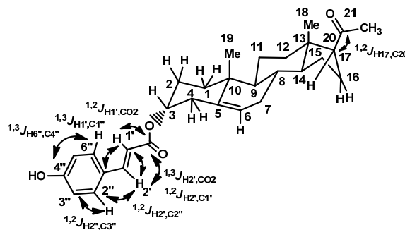
Figure 2. J CH correlations in the HMBC NMR spectrum of compound 17 .
